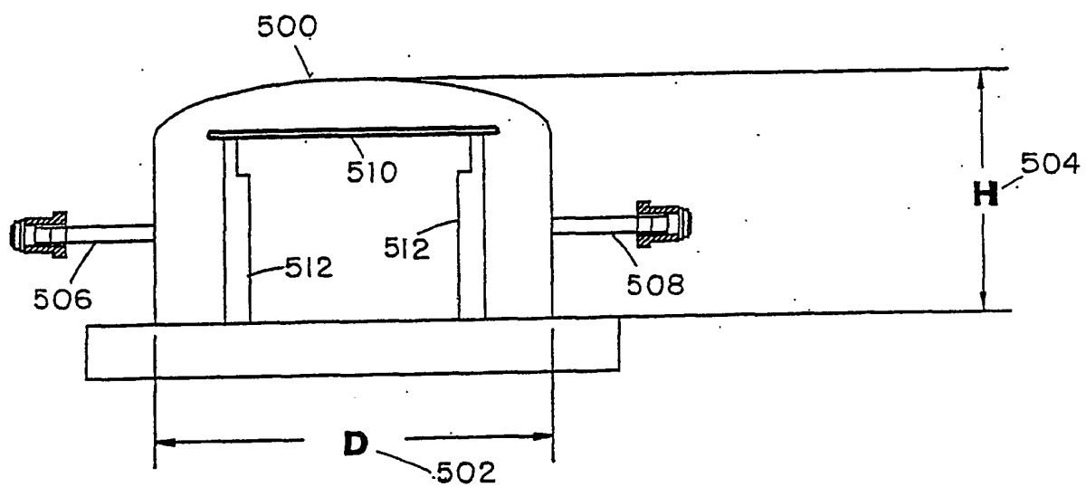
Wafer Chamber
